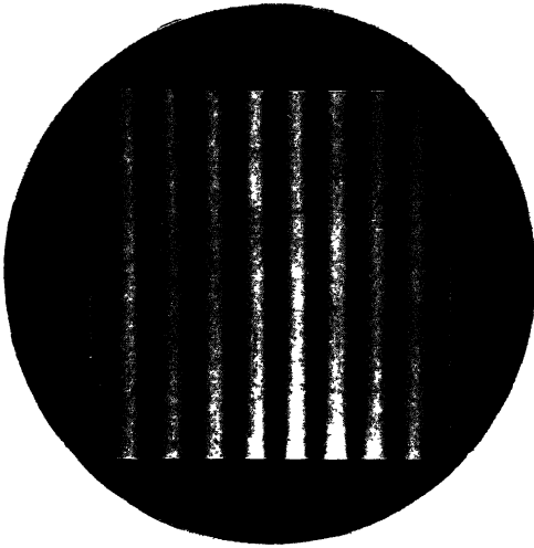
FIG. 132.—Black Central Band and equidistant Spectrum Bands on each side, afforded by Babinet's Composite Plate of two Quartz Wedges, one parallel and the other perpendicular to the Axis. (Direct Photograph of Screen Picture as projected by Lantern Polariscope)
